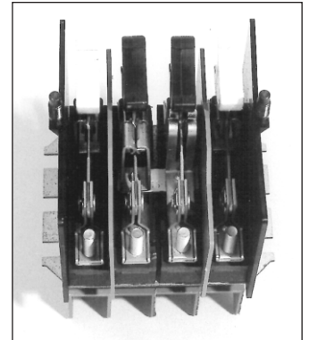
Back-connected types
