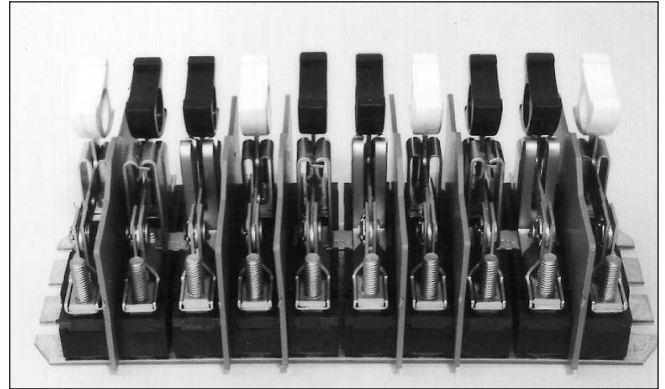
Front-connected type
