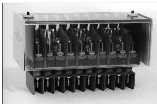
Nonslotted, back-connected clear cover – The nonslotted covers for back-connected switches fit flush with the panel because all wiring exits at the rear of the test switch.
