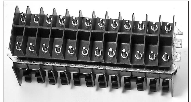
Back-connected types
