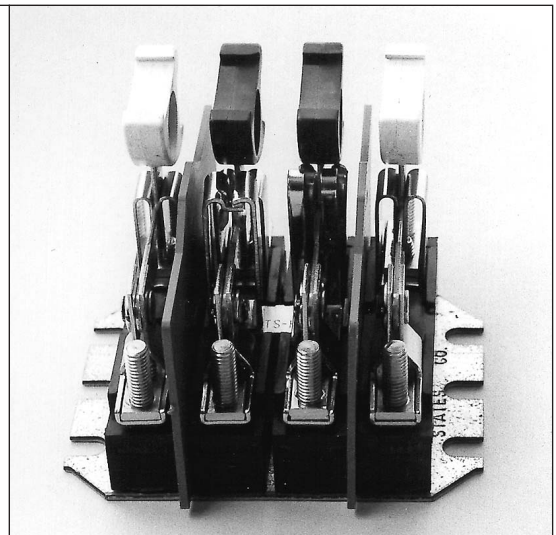
4-Pole Test Switch - Cat. No. 204-N
